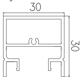
Doga H 30 mm
