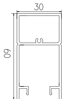
Doga H 60 mm
